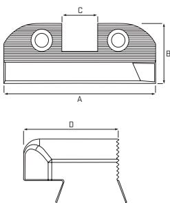
Rear Sight: Square
