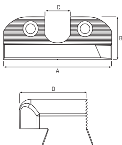
Rear Sight: Round (U)
