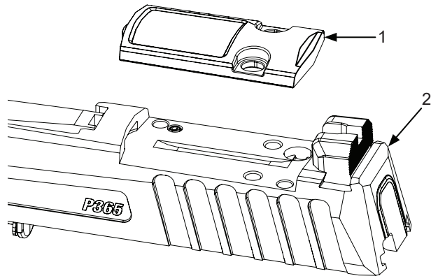
Figure 3. Removal of Sight Plate
