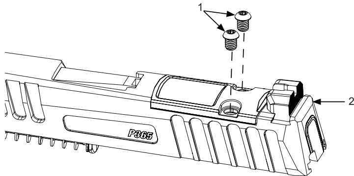
Figure 2. Remove Sight Plate Screw.
