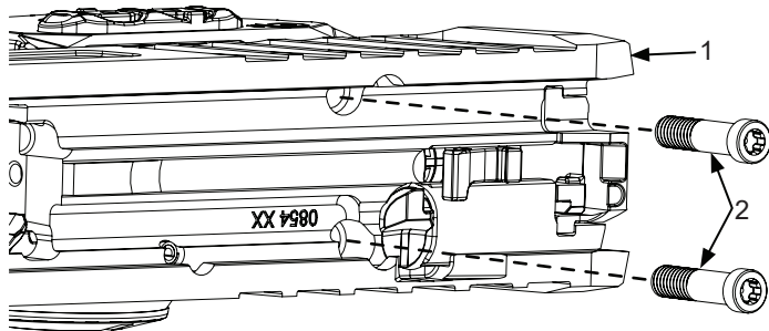
Figure 5. Install Optic Mounting Screws.
