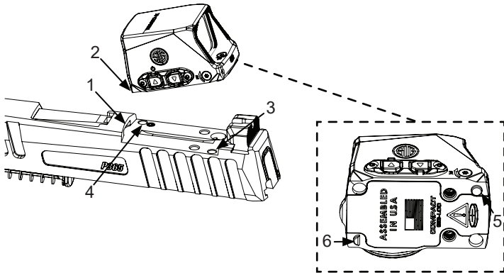
Figure 4. Position Sight on Slide
