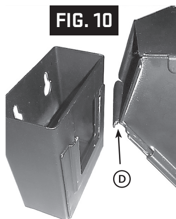
FIG. 10 10. Trap walls will slide down into base mount with Plate D facing down. Entering slots on base mount first. Fig. 11
